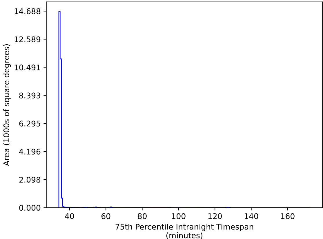
ddf_acor_sf25_lsf30_lsr10_v3.4_10yrs All sky iz bands: 75th Percentile Intranight Timespan
