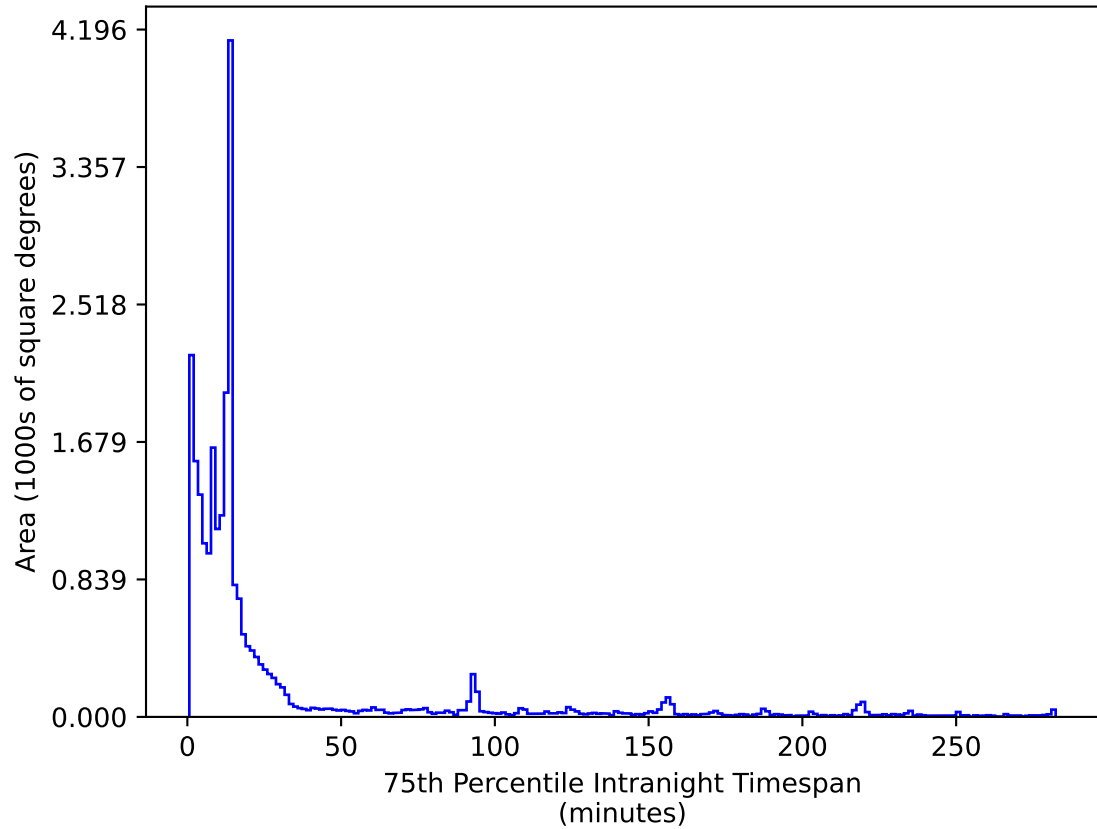
ddf_acor_sf25_lsf30_lsr10_v3.4_10yrs All sky i band: 75th Percentile Intranight Timespan
