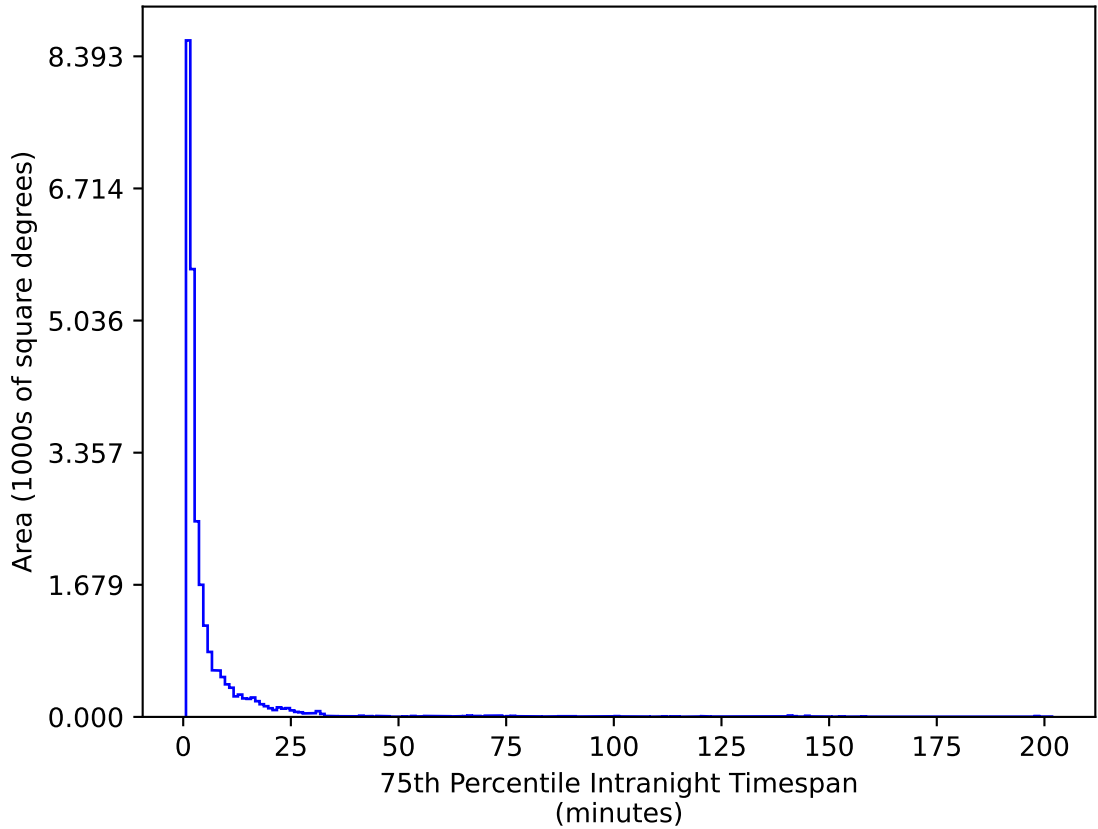
ddf_acor_sf25_lsf30_lsr10_v3.4_10yrs All sky g band: 75th Percentile Intranight Timespan
