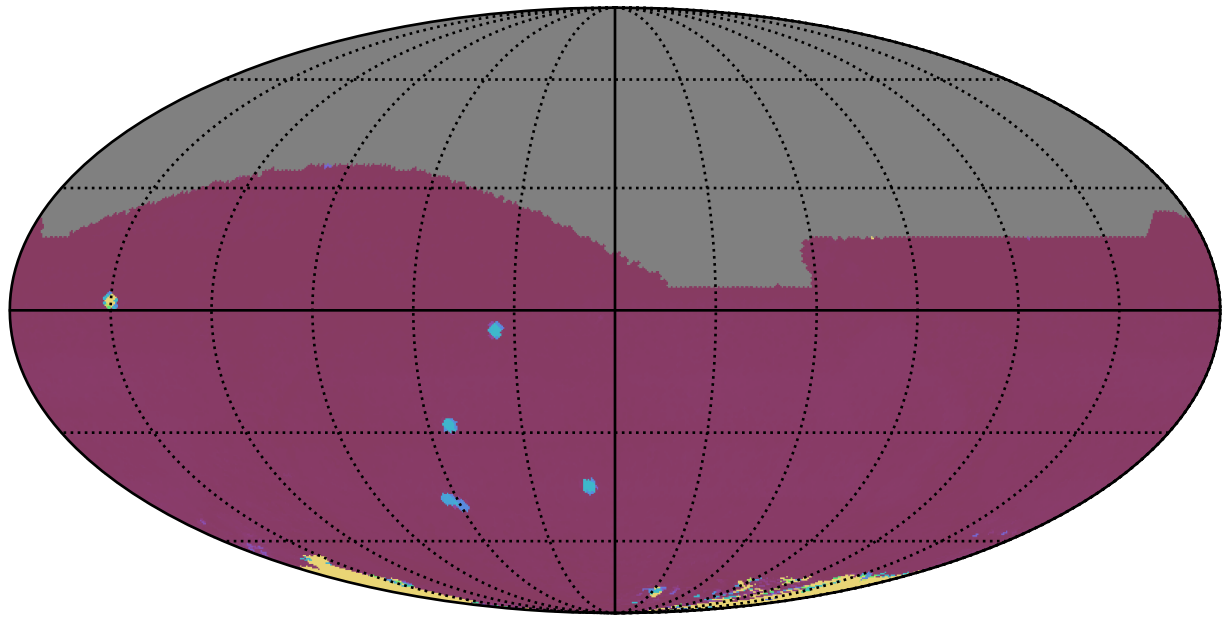
ddf_acor_sf25_lsf30_lsr10_v3.4_10yrs All sky: 75th Percentile Intranight Timespan
