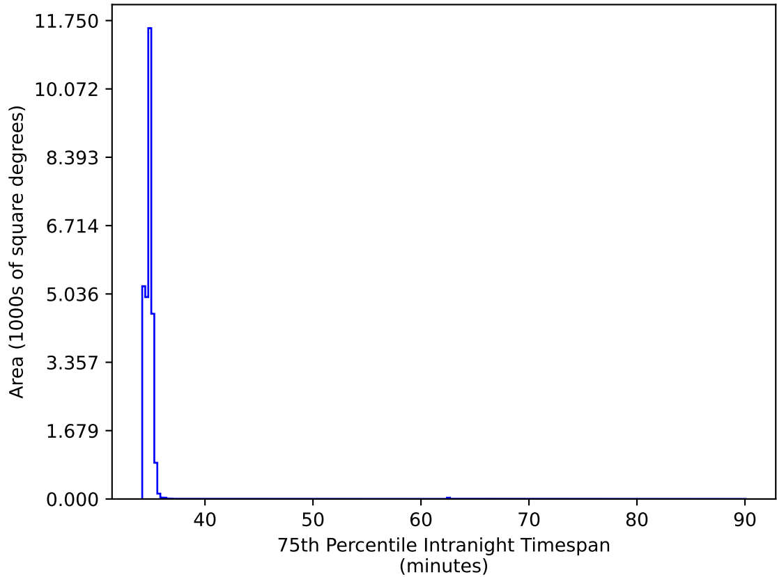
ddf_acor_sf25_lsf30_lsr10_v3.4_10yrs All sky: 75th Percentile Intranight Timespan
