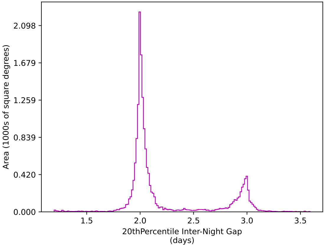
ddf_acor_sf25_lsf30_lsr10_v3.4_10yrs WFD z band: 20thPercentile Inter-Night Gap
