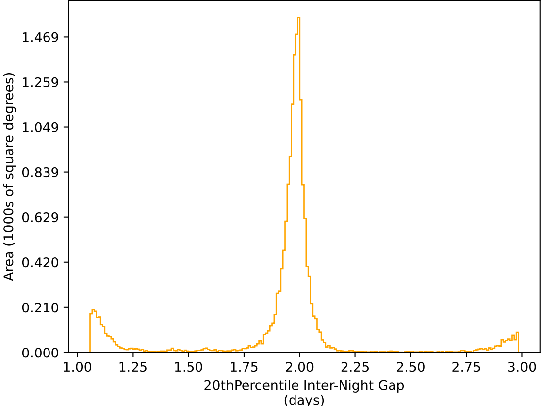
ddf_acor_sf25_lsf30_lsr10_v3.4_10yrs WFD r band: 20thPercentile Inter-Night Gap
