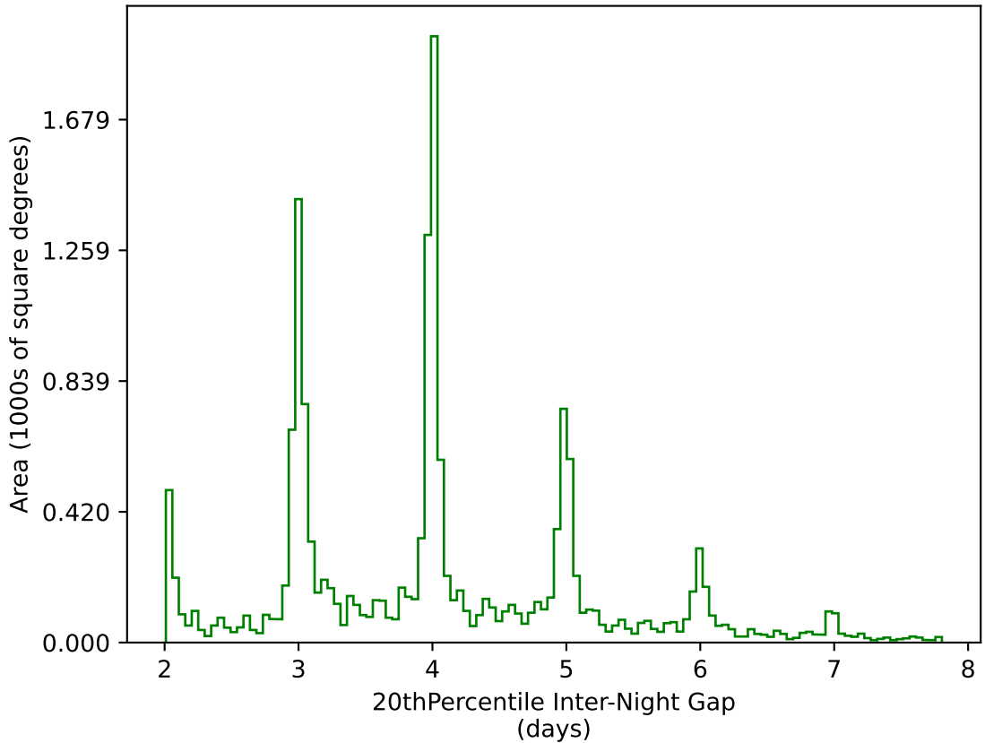
ddf_acor_sf25_ls30_lsr10_v3.4_10yrs WFD g band: 20thPercentile Inter-Night Gap
