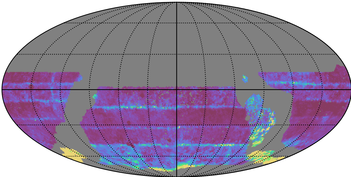
ddf_acor_sf25_lsf30_lsr10_v3.4_10yrs WFD all bands: 20thPercentile Inter-Night Gap
