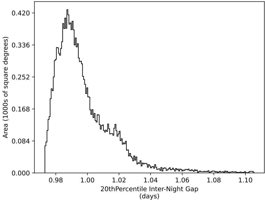
ddf_acor_sf25_lsf30_lsr10_v3.4_10yrs WFD all bands: 20thPercentile Inter-Night Gap
