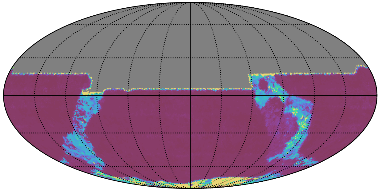
ddf_acor_sf25_lsf30_lsr10_v3.4_10yrs All sky y band: 20thPercentile Inter-Night Gap
