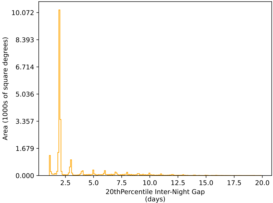
ddf_acor_sf25_lsf30_lsr10_v3.4_10yrs All sky r band: 20thPercentile Inter-Night Gap
