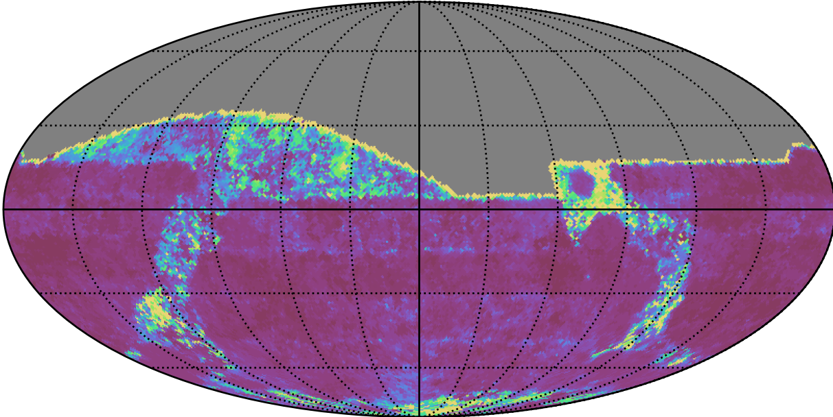
ddf_acor_sf25_lsf30_lsr10_v3.4_10yrs All sky g band: 20thPercentile Inter-Night Gap
