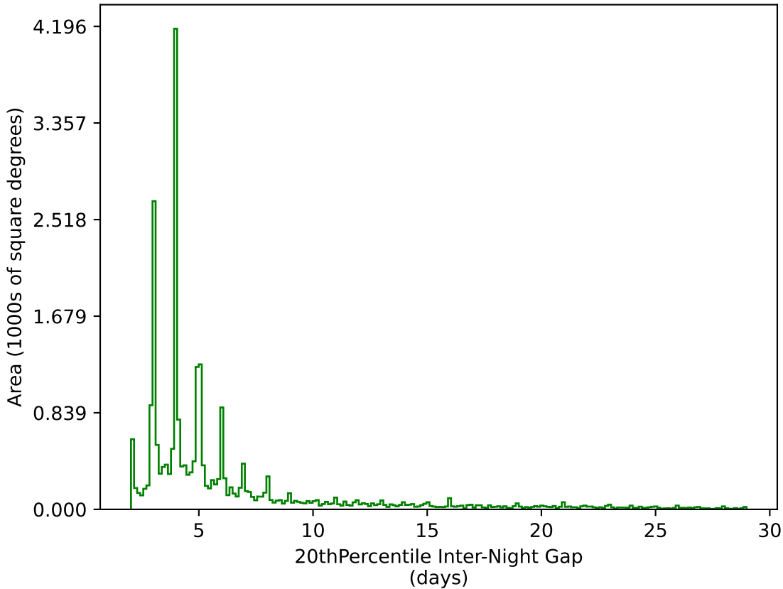
ddf_acor_sf25_lsf30_lsr10_v3.4_10yrs All sky g band: 20thPercentile Inter-Night Gap
