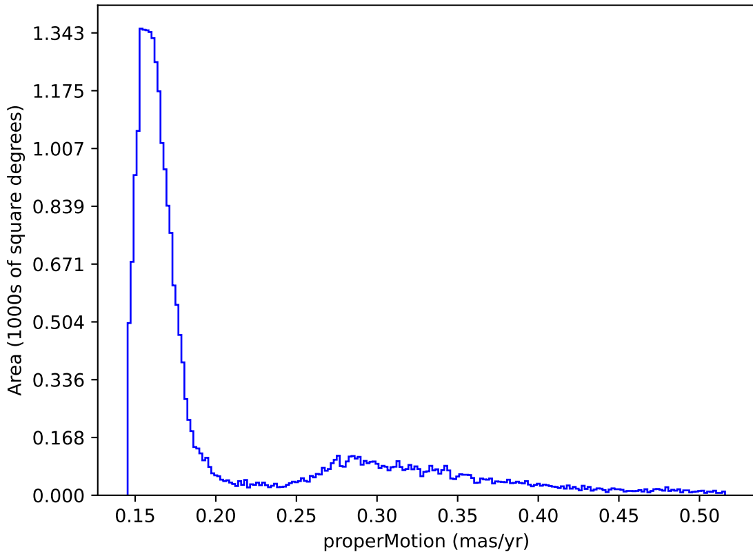
ddf_acor_sf25_lsf30_lsr10_v3.4_10yrs : properMotion
