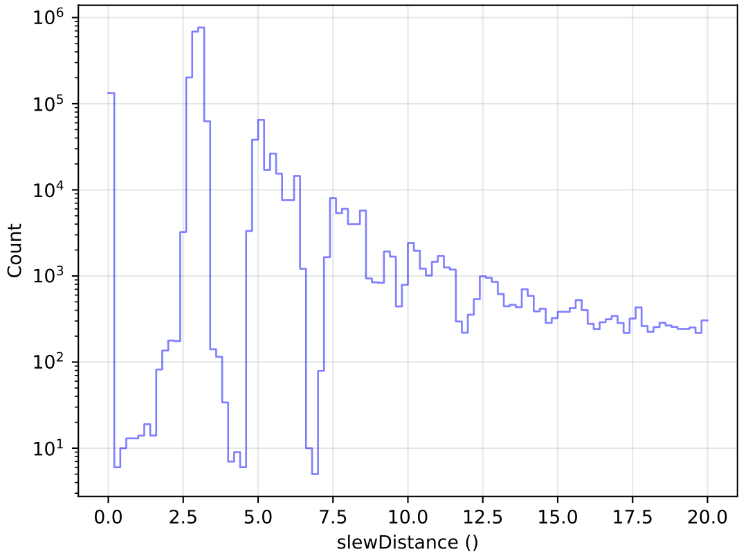
ddf_acor_sf25_lsf30_lsr10_v3.4_10yrs All visits: Zoom Slew Distance Histogram
