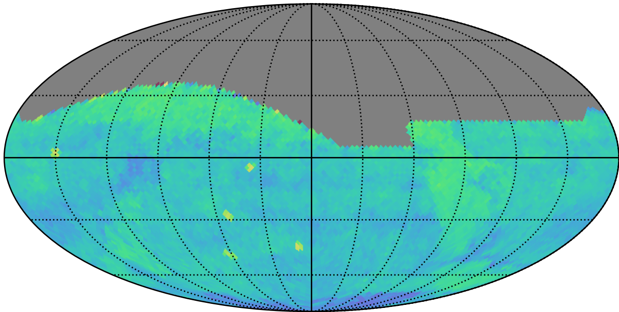
ddf_acor_sf25_lsf30_lsr10_v3.4_10yrs (g or r or i): PairFraction
