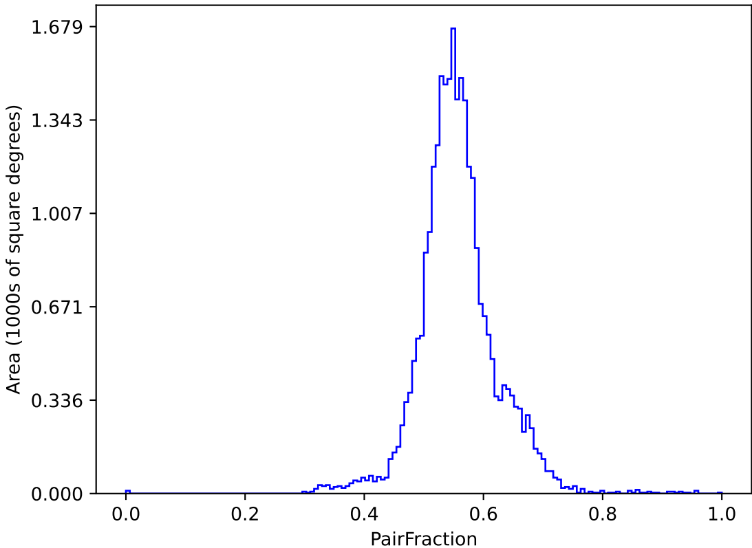
ddf_acor_sf25_lsf30_lsr10_v3.4_10yrs (g or r or i): PairFraction
