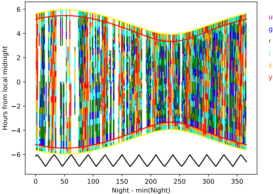
ddf_acor_sf25_lsf30_lsr10_v3.4_10yrs year 9-10: Hourglass
