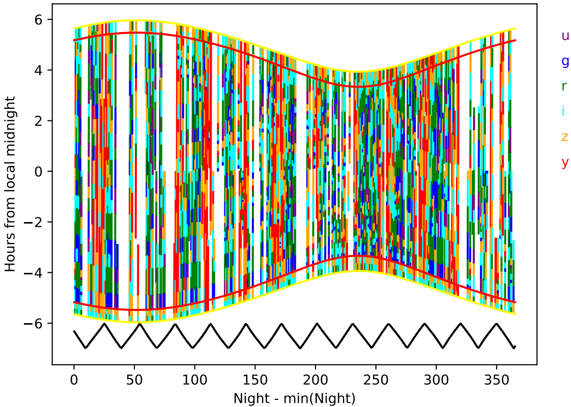
ddf_acor_sf25_lsf30_lsr10_v3.4_10yrs year 7-8: Hourglass
