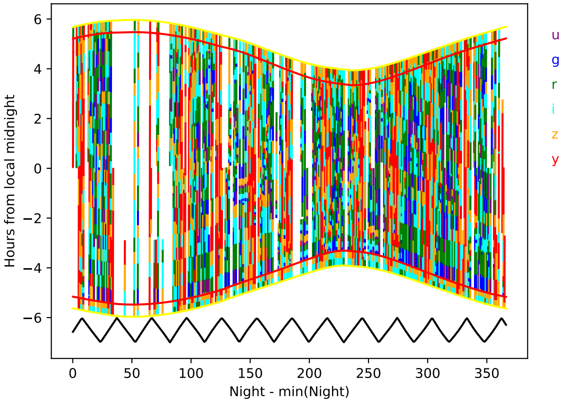
ddf_acor_sf25_lsf30_lsr10_v3.4_10yrs year 3-4: Hourglass
