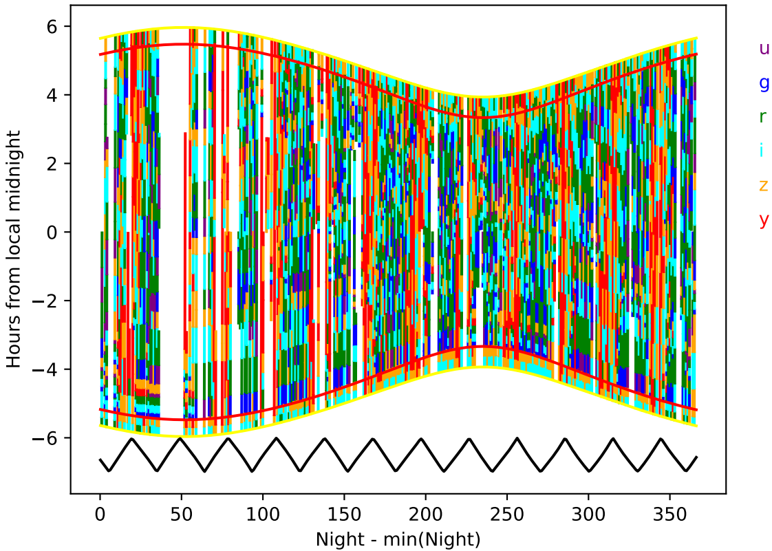
ddf_acor_sf25_lsf30_lsr10_v3.4_10yrs year 2-3: Hourglass
