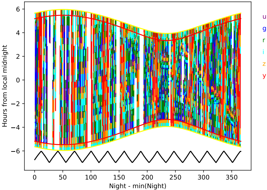
ddf_acor_sf25_lsf30_lsr10_v3.4_10yrs year 0-1: Hourglass
