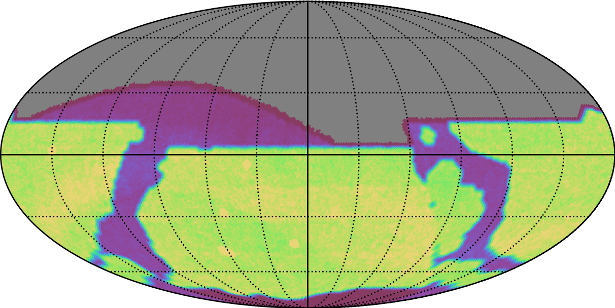
ddf_acor_sf25_lsf30_lsr10_v3.4_10yrs : Count observationStartMJD
