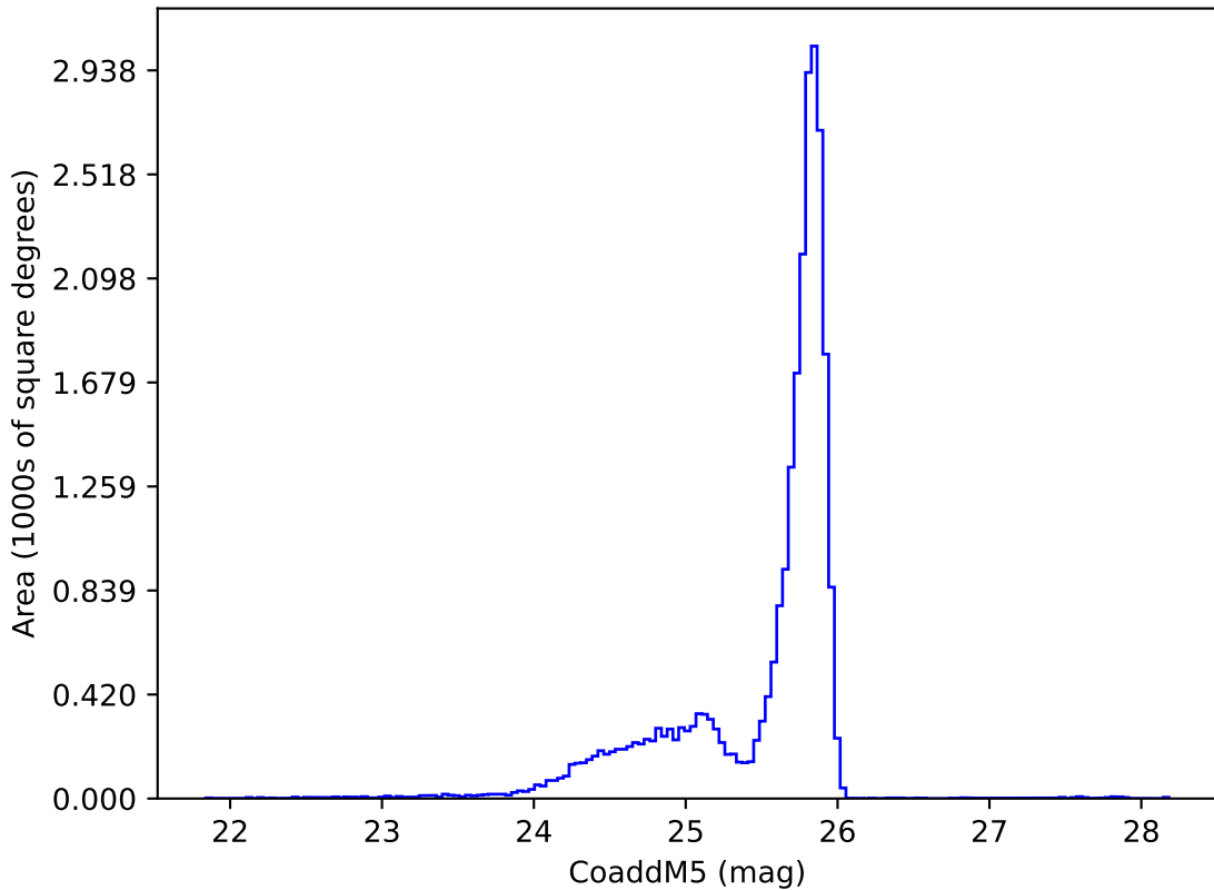
ddf_acor_sf25_lsf30_lsr10_v3.4_10yrs z: CoaddM5
