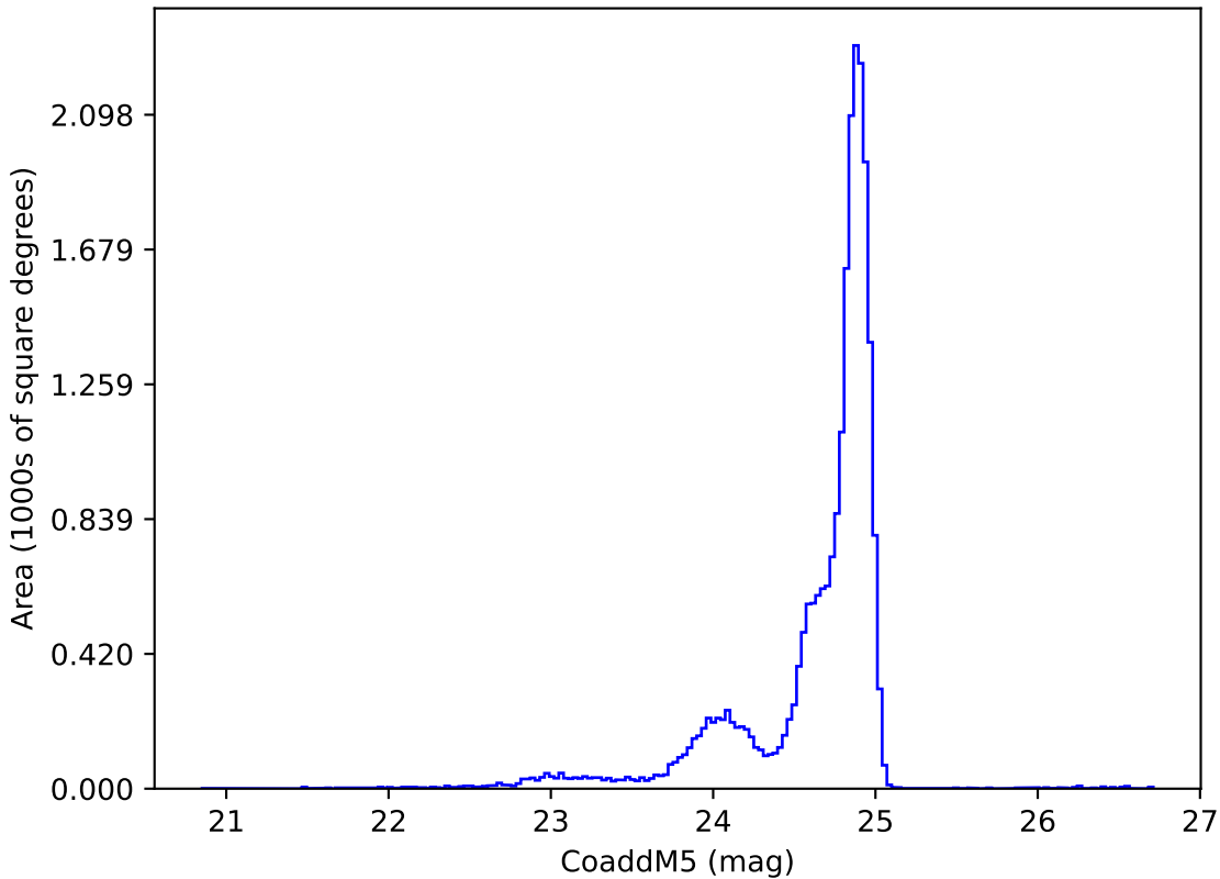
ddf_acor_sf25_lsf30_lsr10_v3.4_10yrs y: CoaddM5
