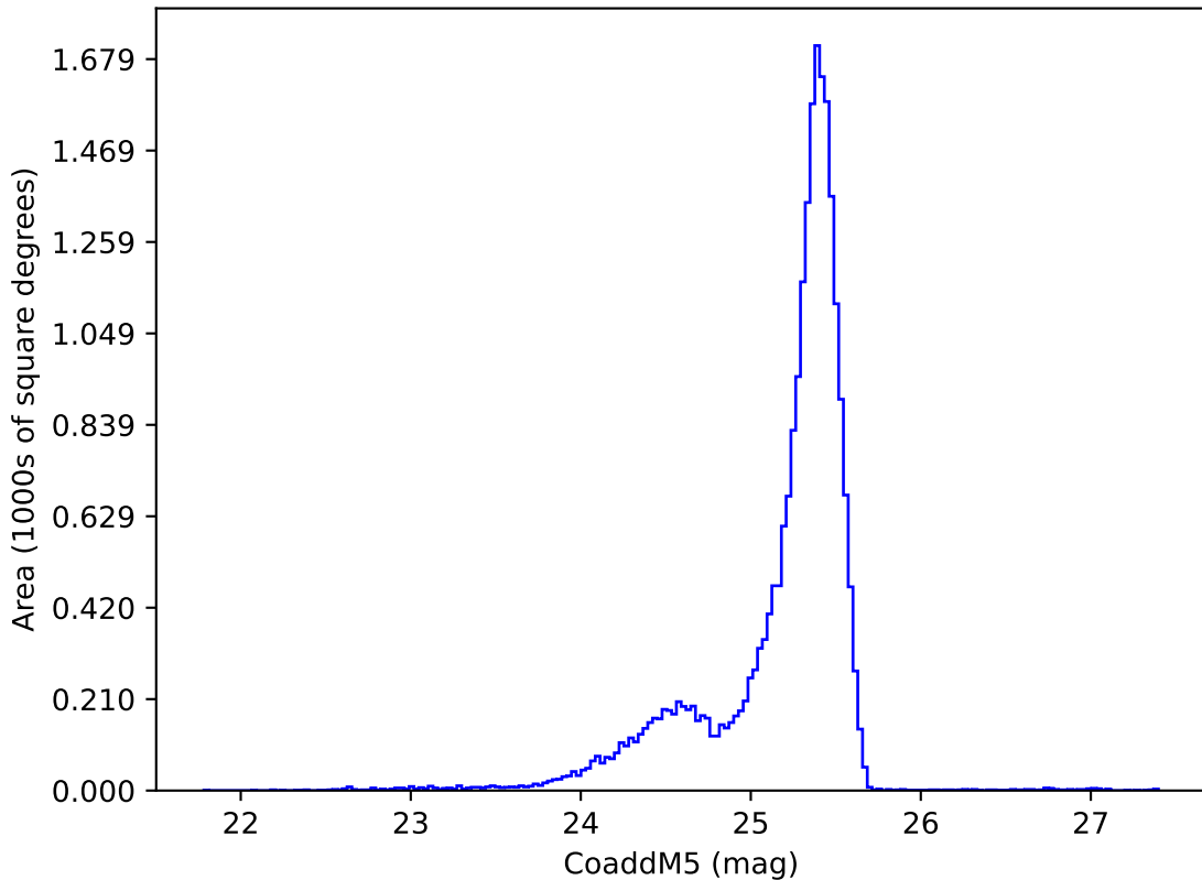
ddf_acor_sf25_ls30_lsr10_v3.4_10yrs u: CoaddM5
