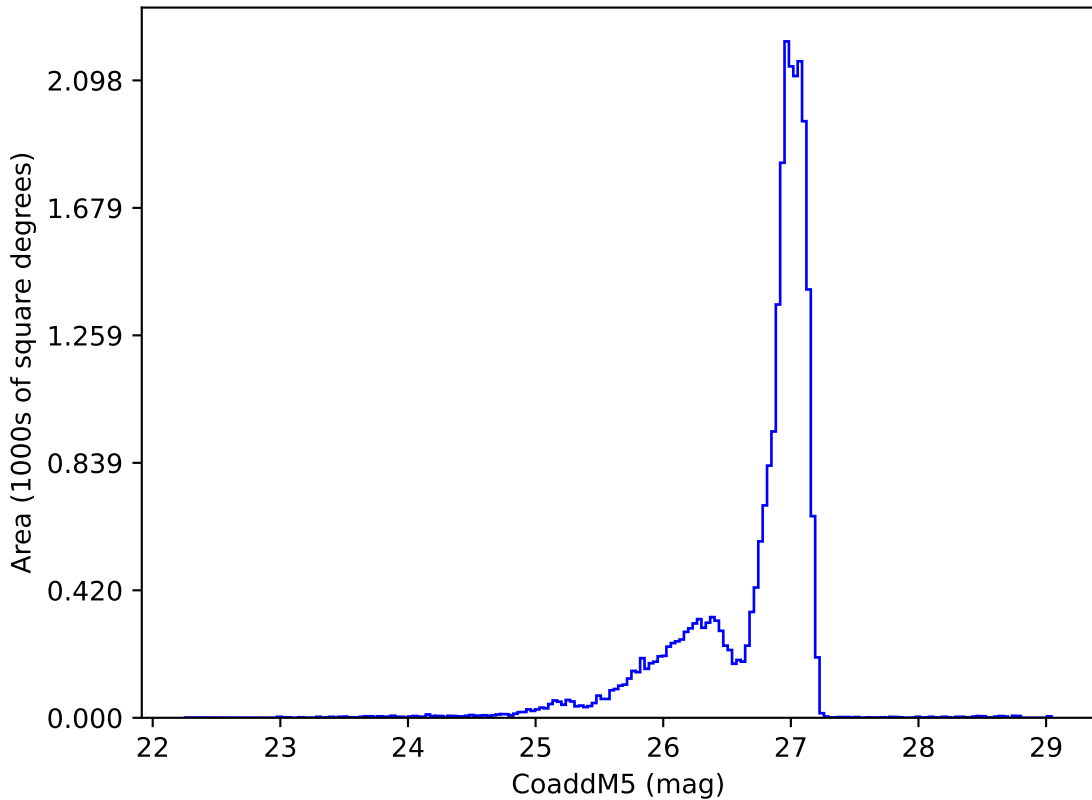
ddf_acor_sf25_lsf30_lsr10_v3.4_10yrs r: CoaddM5
