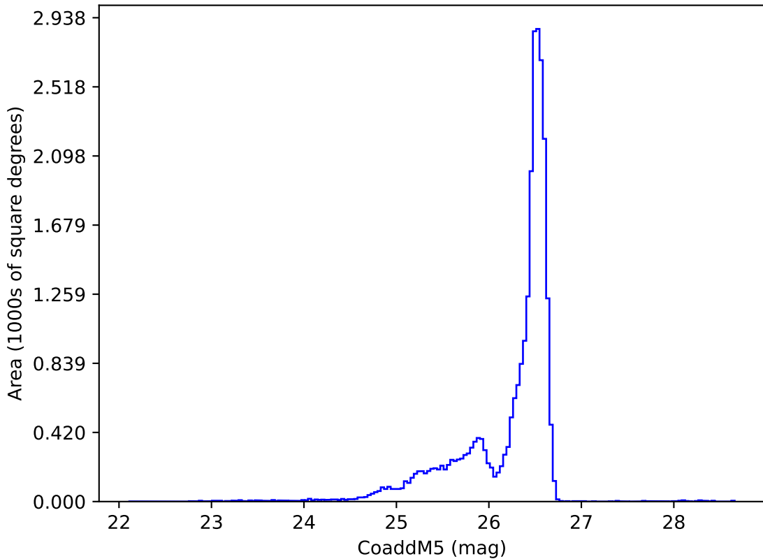
ddf_acor_sf25_lsf30_lsr10_v3.4_10yrs i: CoaddM5
