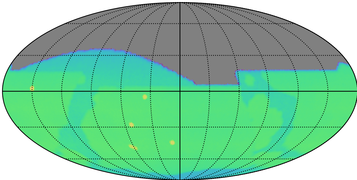
ddf_acor_sf25_lsf30_lsr10_v3.4_10yrs : CoaddM5
