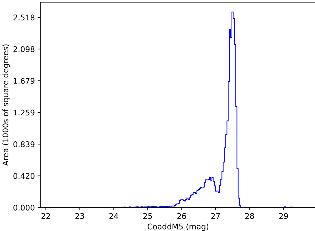
ddf_acor_sf25_lsf30_lsr10_v3.4_10yrs : CoaddM5
