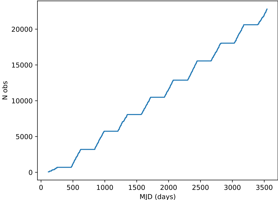
ddf_acor_sf25_lsf30_lsr10_v3.4_10yrs all bands: DD:XMM_LSS Cumulative NVisits
