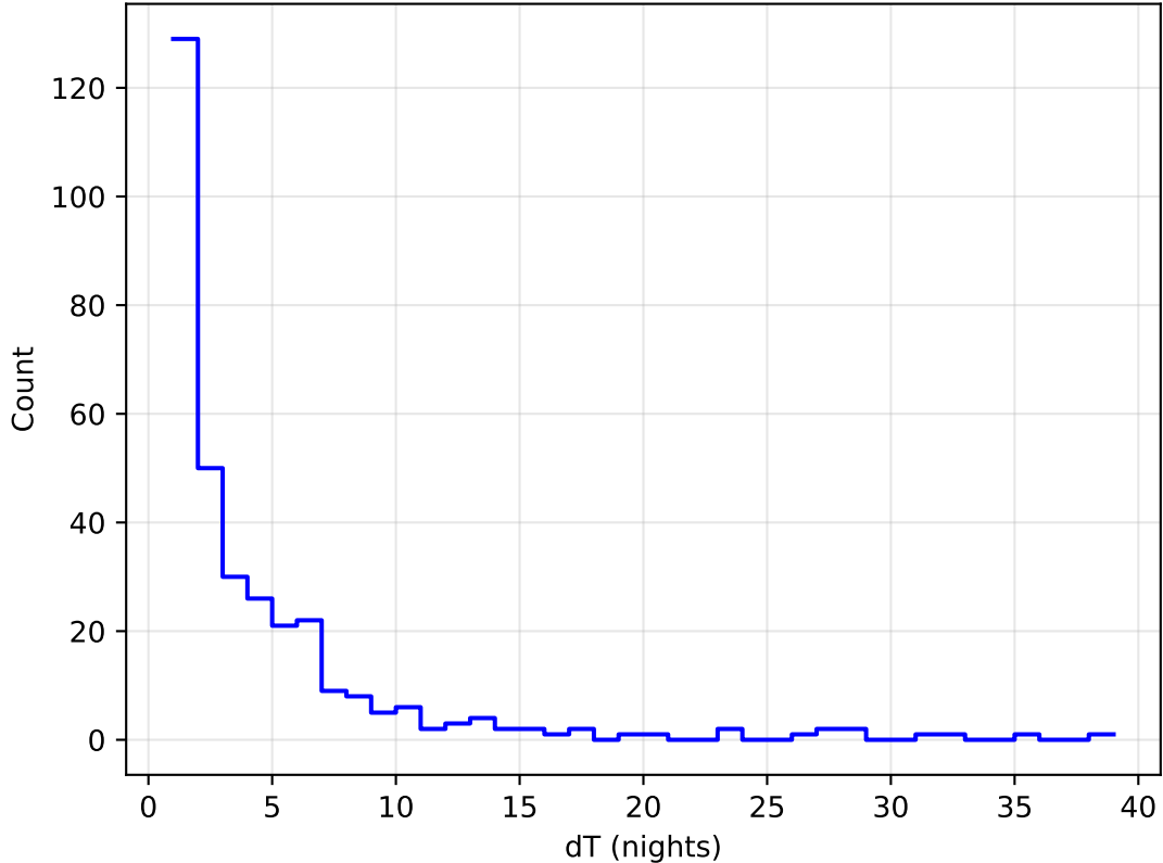
ddf_acor_sf25_lsf30_lsr10_v3.4_10yrs all bands: DD:WFD Delta Nights Histogram
