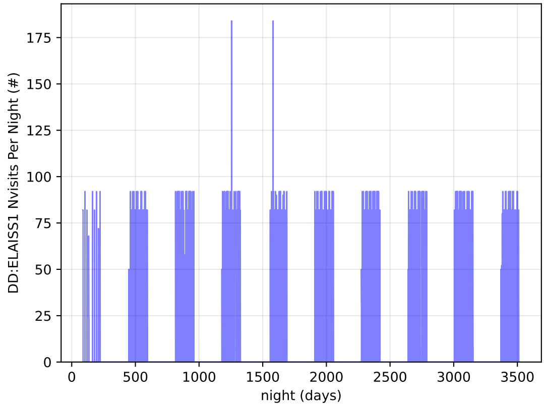
ddf_acor_sf25_lsf30_lsr10_v3.4_10yrs all bands: DD:ELAISS1 Nvisits Per Night
