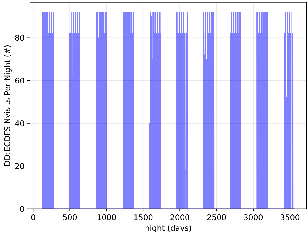
ddf_acor_sf25_lsf30_lsr10_v3.4_10yrs all bands: DD:ECDFS Nvisits Per Night
