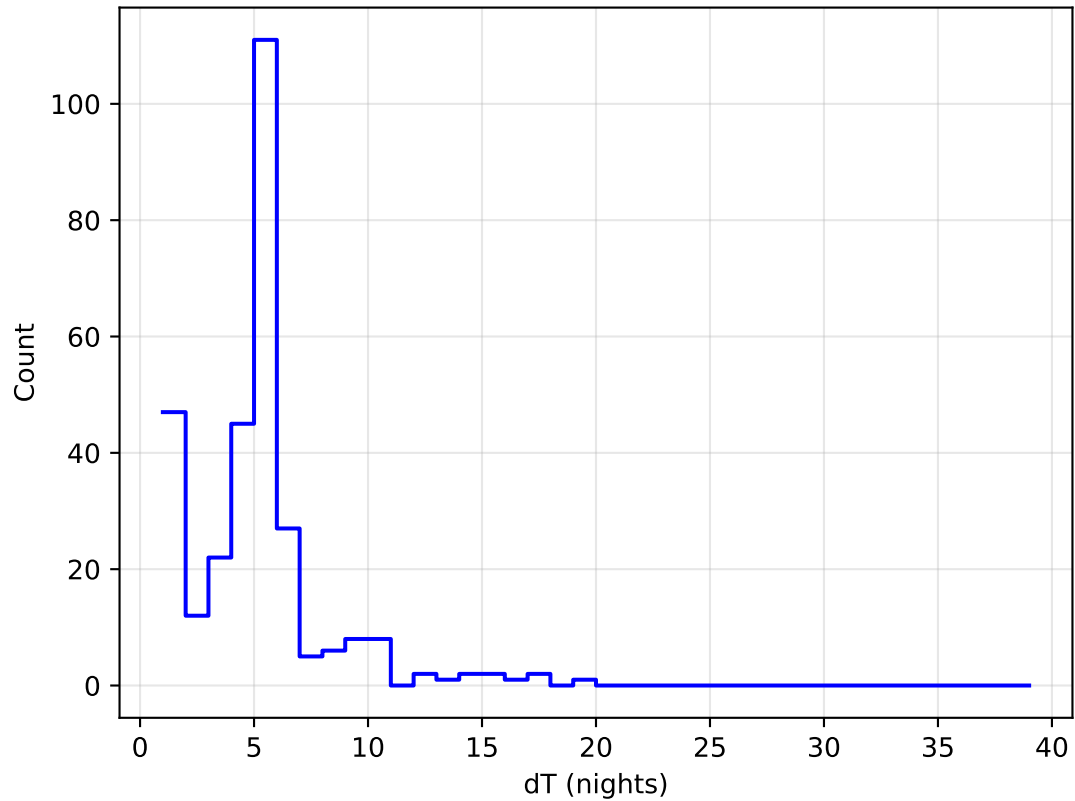
ddf_acor_sf25_lsf30_lsr10_v3.4_10yrs all bands: DD:ECDFS Delta Nights Histogram
