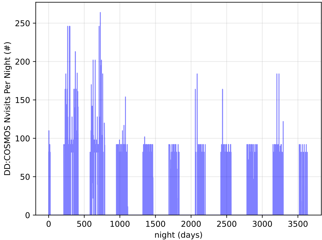
ddf_acor_sf25_lsf30_lsr10_v3.4_10yrs all bands: DD: COSMOS Nvisits Per Night
