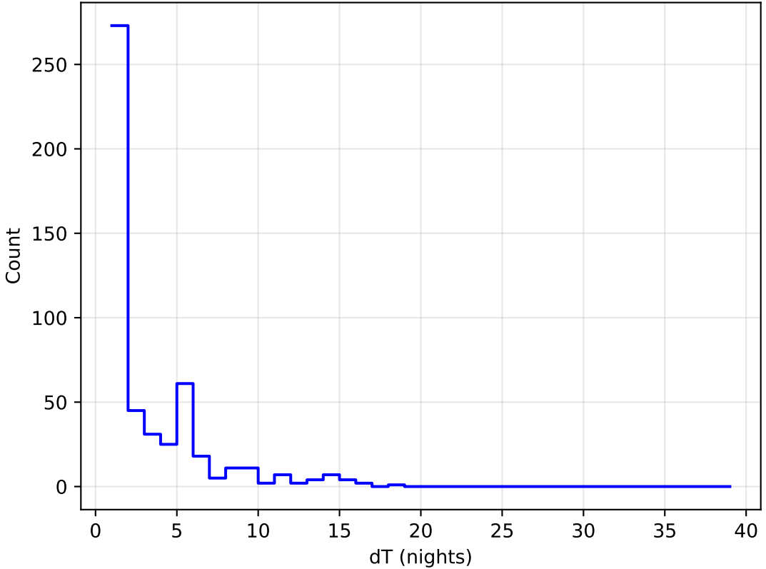
ddf_acor_sf25_Isf30_Isr10_v3.4_10yrs all bands: DD: COSMOS Delta Nights Histogram
