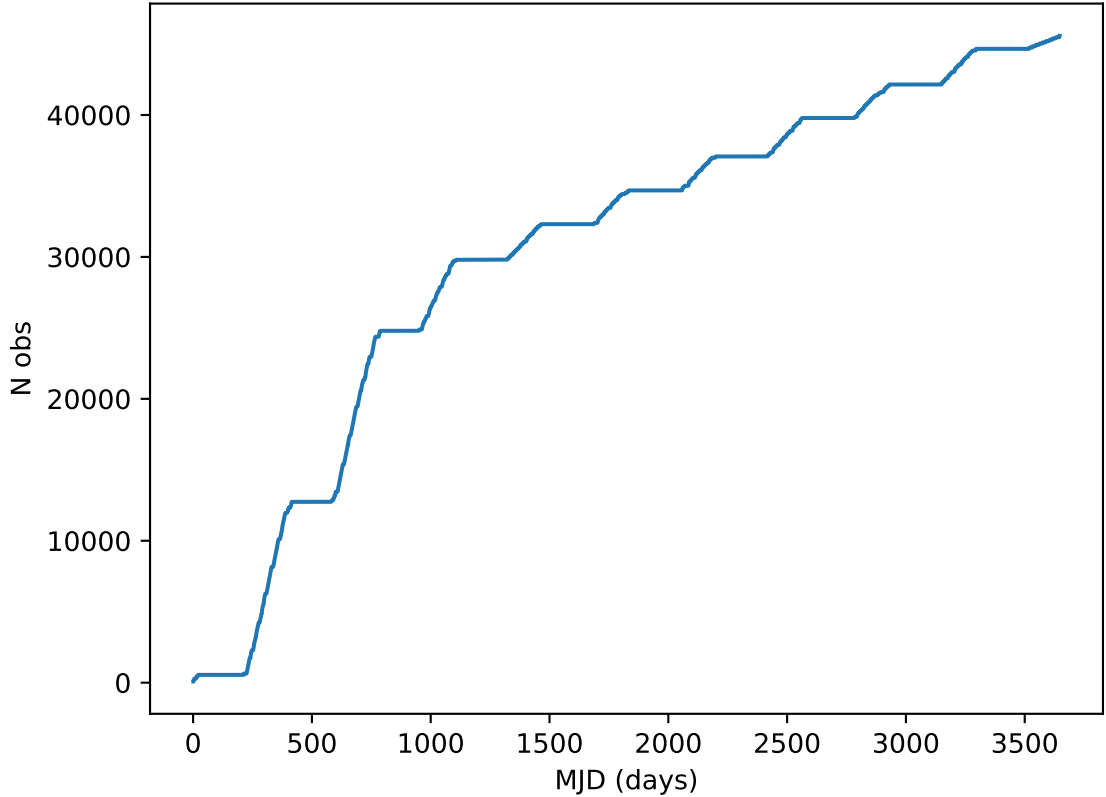
ddf_acor_sf25_lsf30_lsr10_v3.4_10yrs all bands: DD: COSMOS Cumulative NVisits
