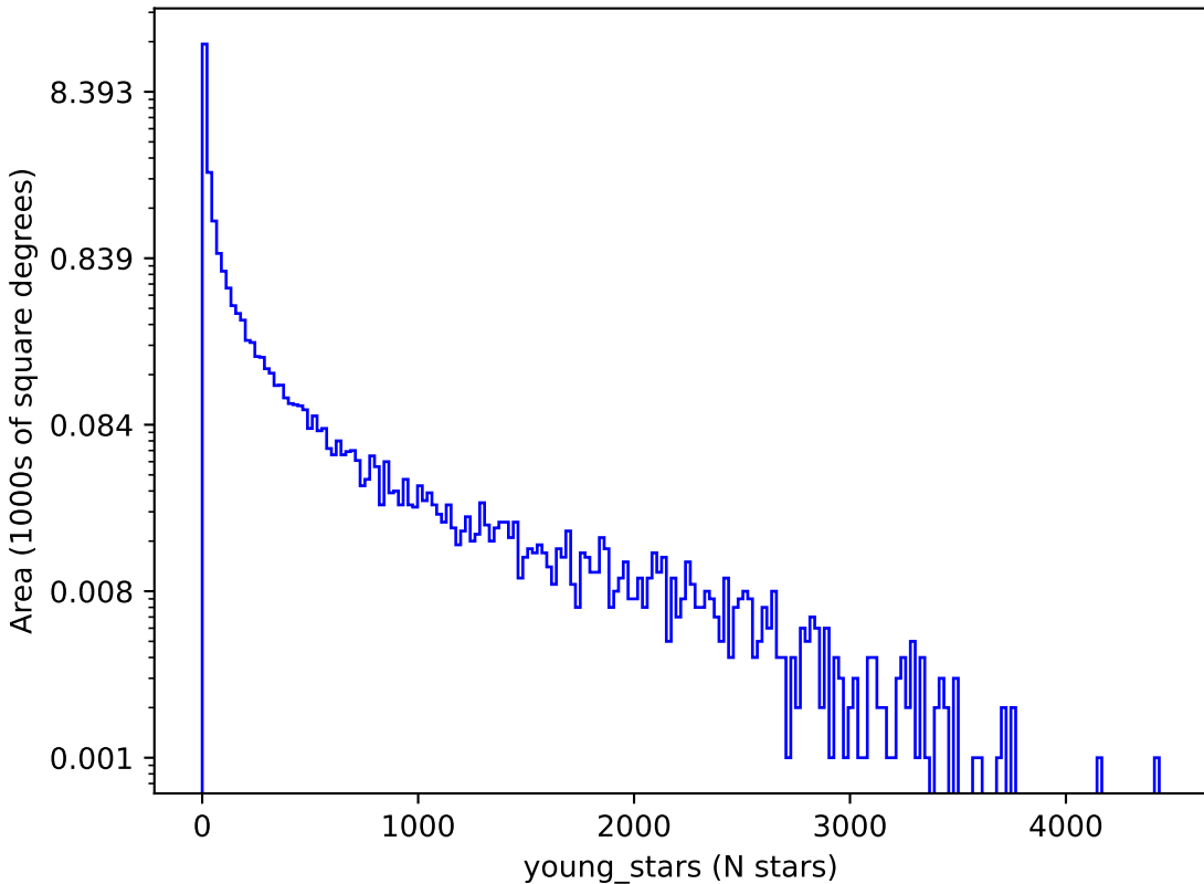
ddf_acor_sf20_lsf40_lsr50_v3.4_10yrs : young_stars
