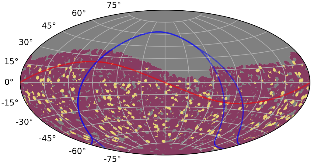
ddf_acor_sf20_lsf40_lsr50_v3.4_10yrs : TDEsPopMetric_some_color
