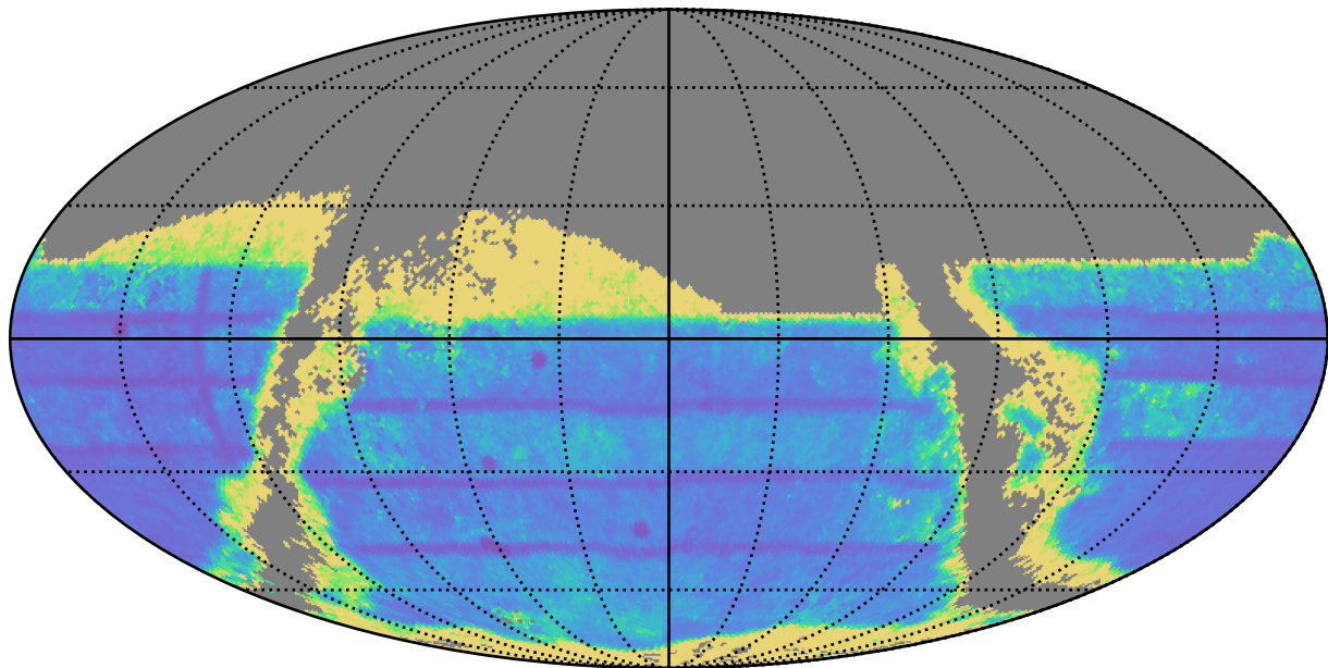
ddf_acor_sf20_lsf40_lsr50_v3.4_10yrs : TDC_precision
