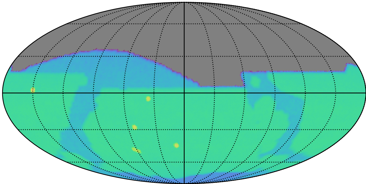
ddf_acor_sf20_lsf40_lsr50_v3.4_10yrs i: SurfaceBrightLimit
