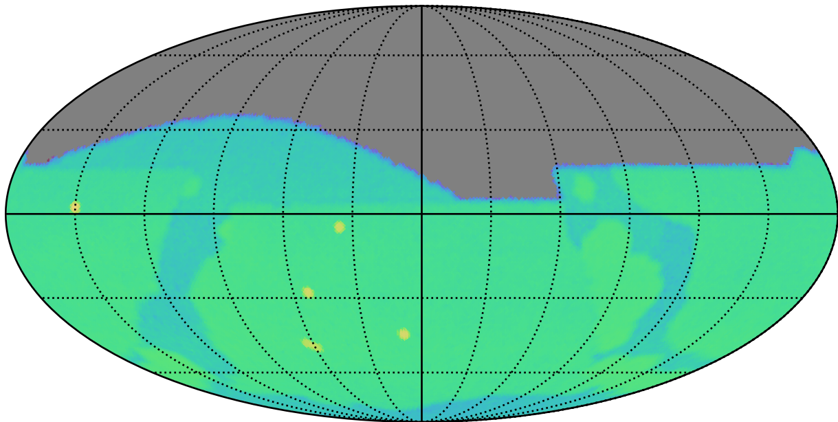
ddf_acor_sf20_lsf40_lsr50_v3.4_10yrs g: SurfaceBrightLimit
