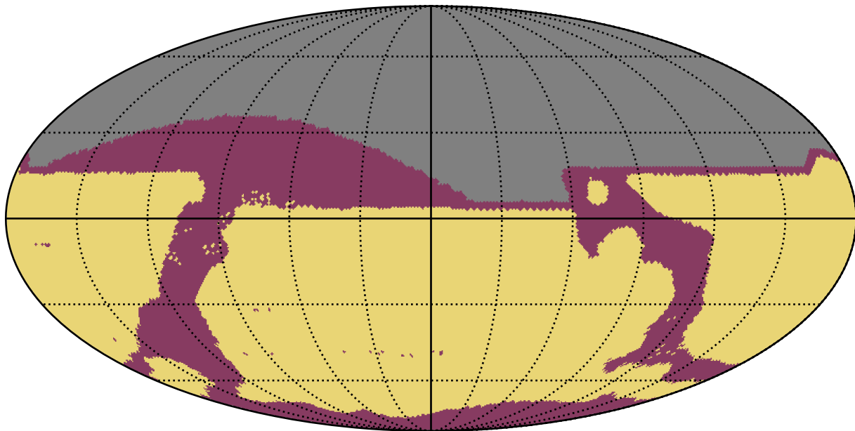
ddf_acor_sf20_lsf40_lsr50_v3.4_10yrs : RapidRevisits
