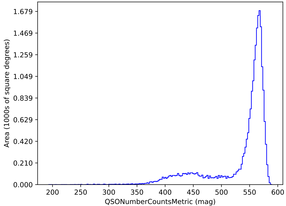
ddf_acor_sf20_lsf40_lsr50_v3.4_10yrs y band and non-DD: QSONumberCountsMetric
