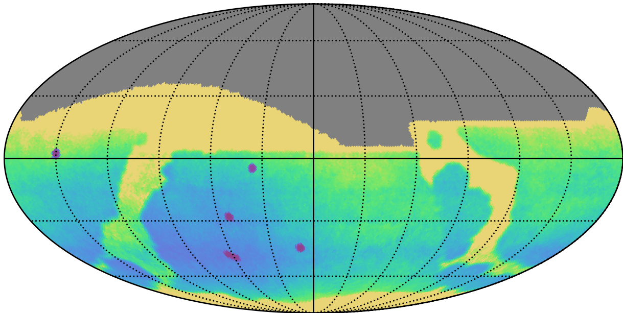
ddf_acor_sf20_lsf40_lsr50_v3.4_10yrs : Parallax Uncert @ 24.0
