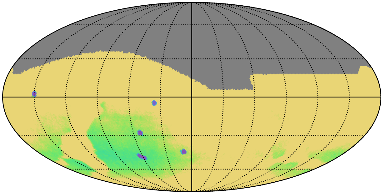
ddf_acor_sf20_lsf40_lsr50_v3.4_10yrs : Parallax Uncert @ 22.4
