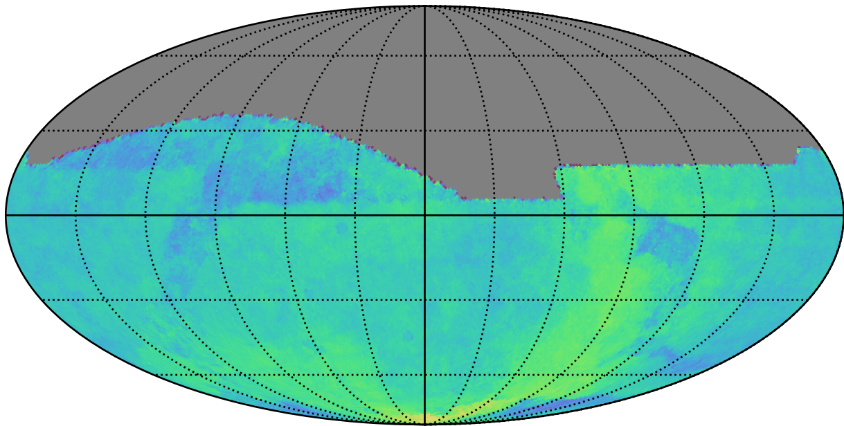
ddf_acor_sf20_lsf40_lsr50_v3.4_10yrs : Parallax Coverage @ 24.0
