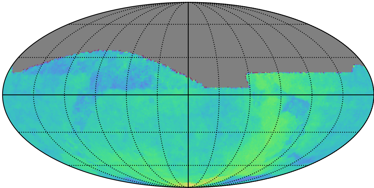
ddf_acor_sf20_lsf40_lsr50_v3.4_10yrs : Parallax Coverage @ 22.4
